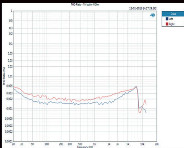
The Total Harmonic Distortion (THD) of the amplifier is below 0.005% across the audio bandwidth 20-20 kHz measured at 1W output power into 4Ω. At 30W output power the amplifier meets THD levels between 0.015% and 0.03% successfully independent of frequency.
