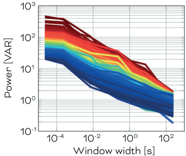
There is a 10x peak to average power ratio for normal music, and with 250 Watts for up to 5 seconds the RUBICON C amplifier has more power than most amplifiers.
