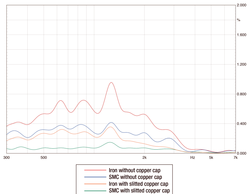
Generic example on 3rd order distortion. This graph shows the effect on a RUBICON 8 woofer, which, with only minor details, is much alike the woofer on RUBICON 6 C.
