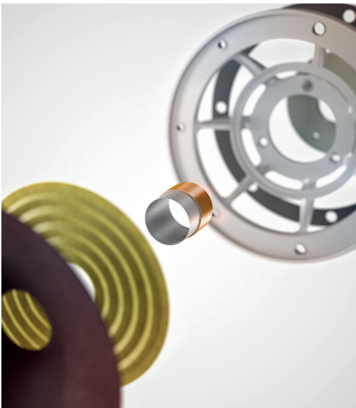
Exploded view of voice coil in RUBICON woofer
